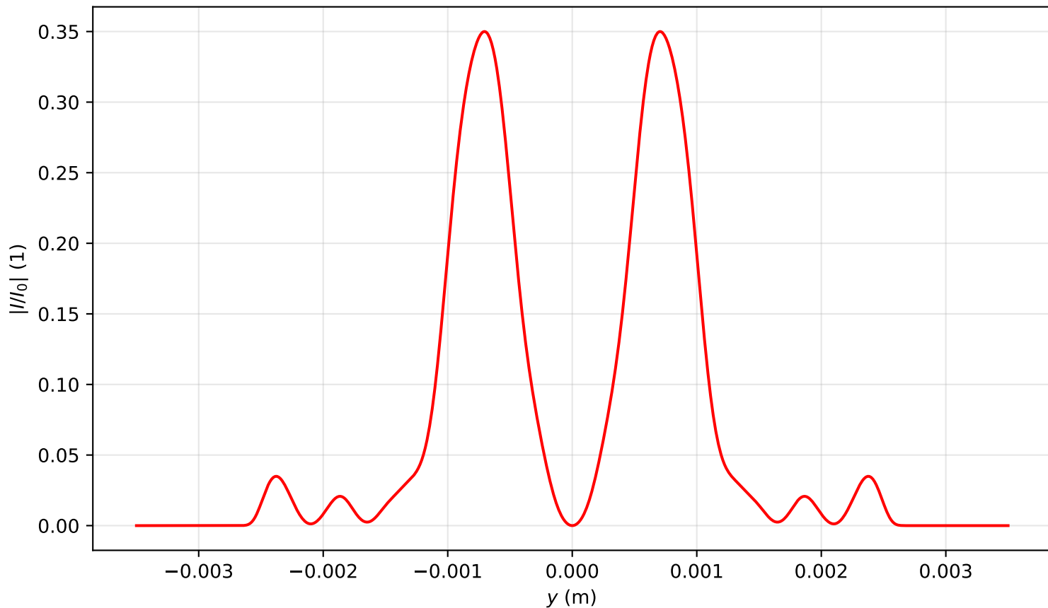
Intensity profile I(x=0, y, z=3.105)/I_0 , P_{in}=6.0P_{cr} , artificial time
